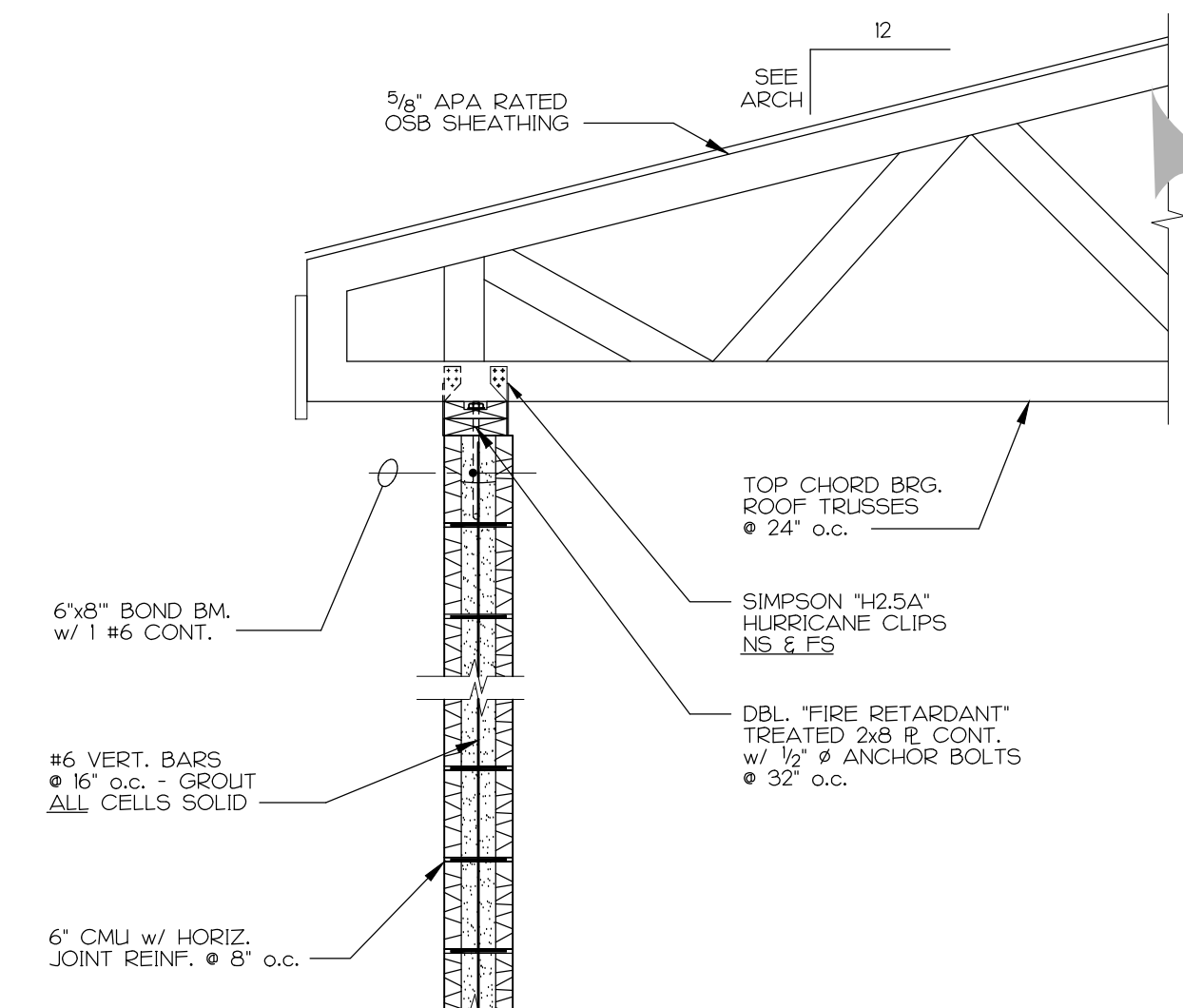
4 SECTION AT STAIR ROOF S8.2 3/4" = 1'-0"
