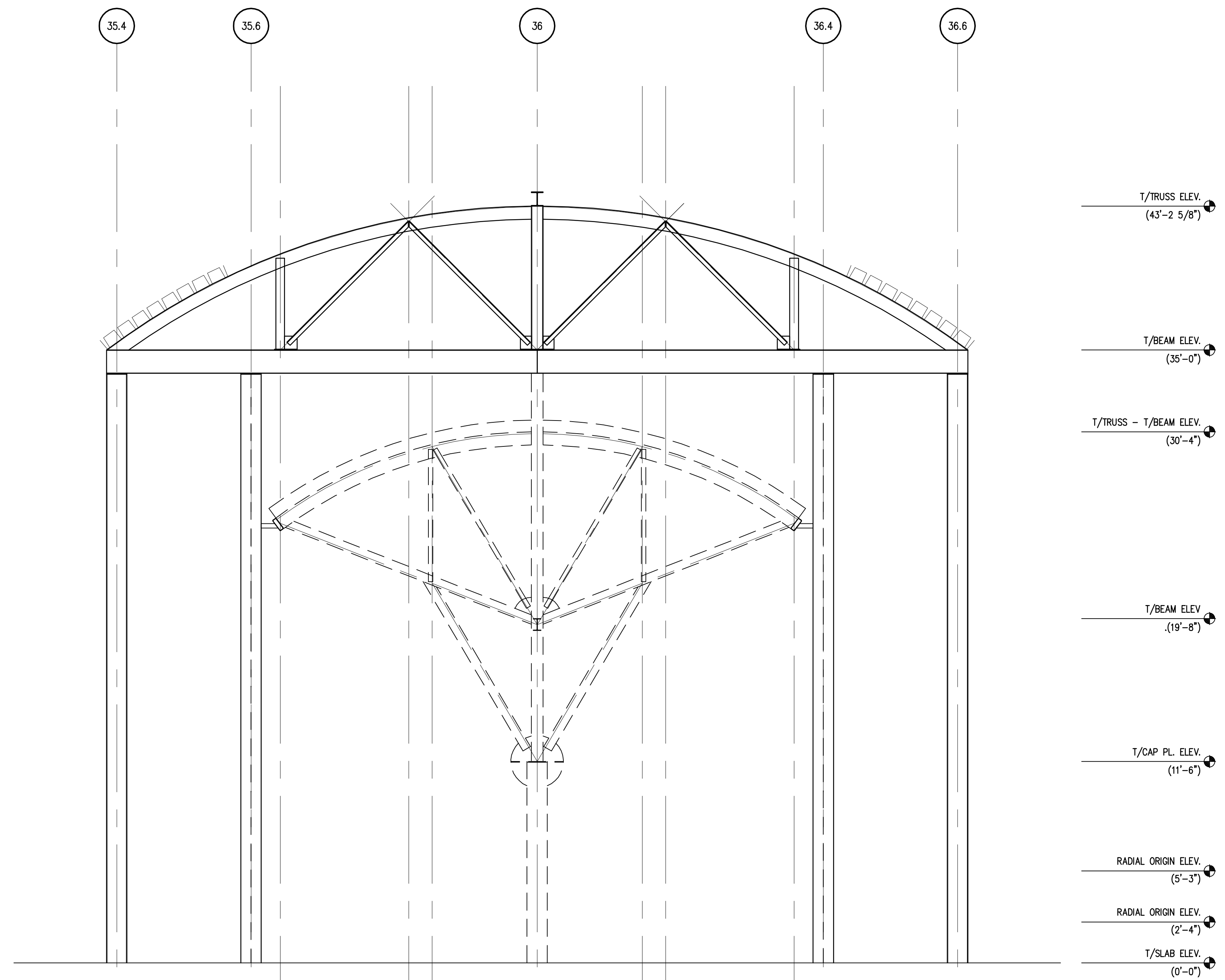
2 PARTIAL SECTION SCALE: 1/4"=1'-0"
