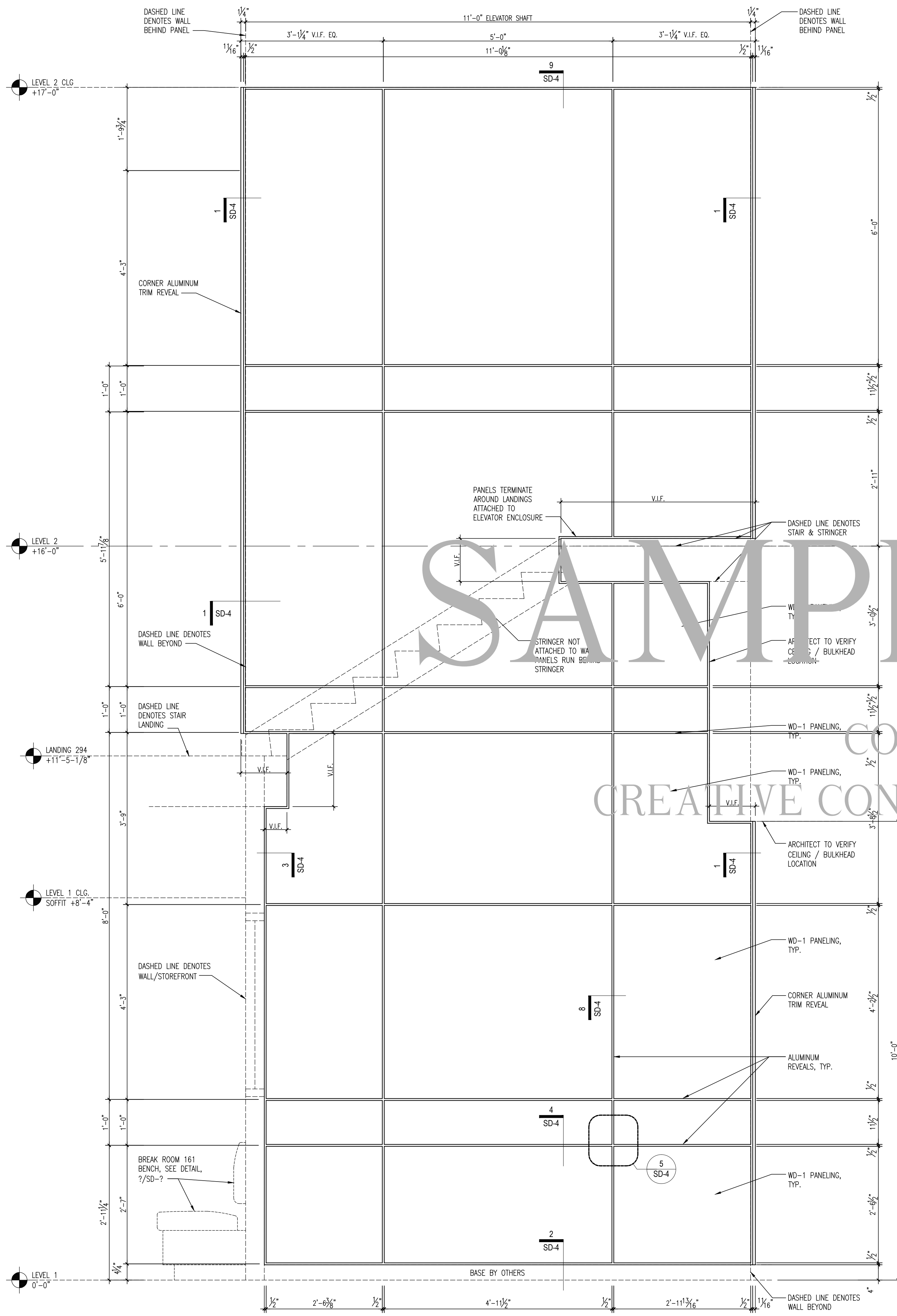
1 ELEVATION @ STAIR - 192 & 193 SD-3 SCALE: 3/4" = 1'-0" 1 THUS
