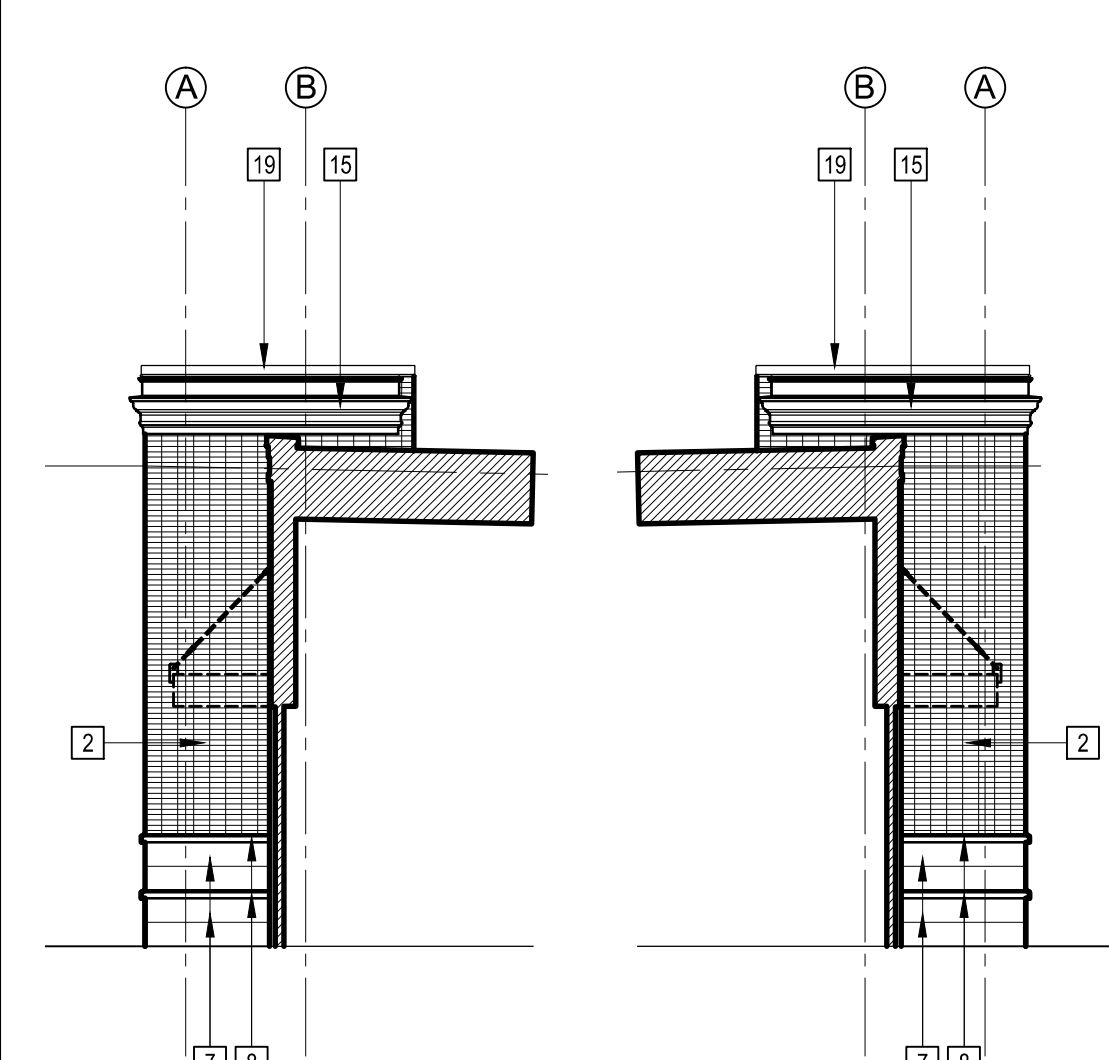
7 ELEVATIONS @ RETURNS 1/8"=1'-0"
