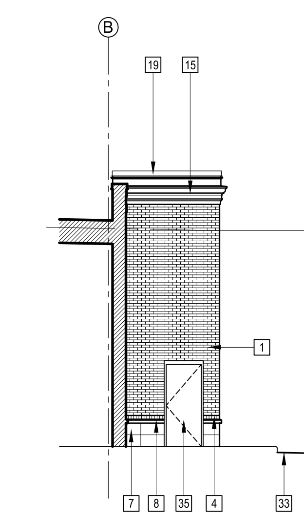
6 SPRINKLER RISER RM. BLDG A NORTH ELEVATION 1/8"=1'-0"
