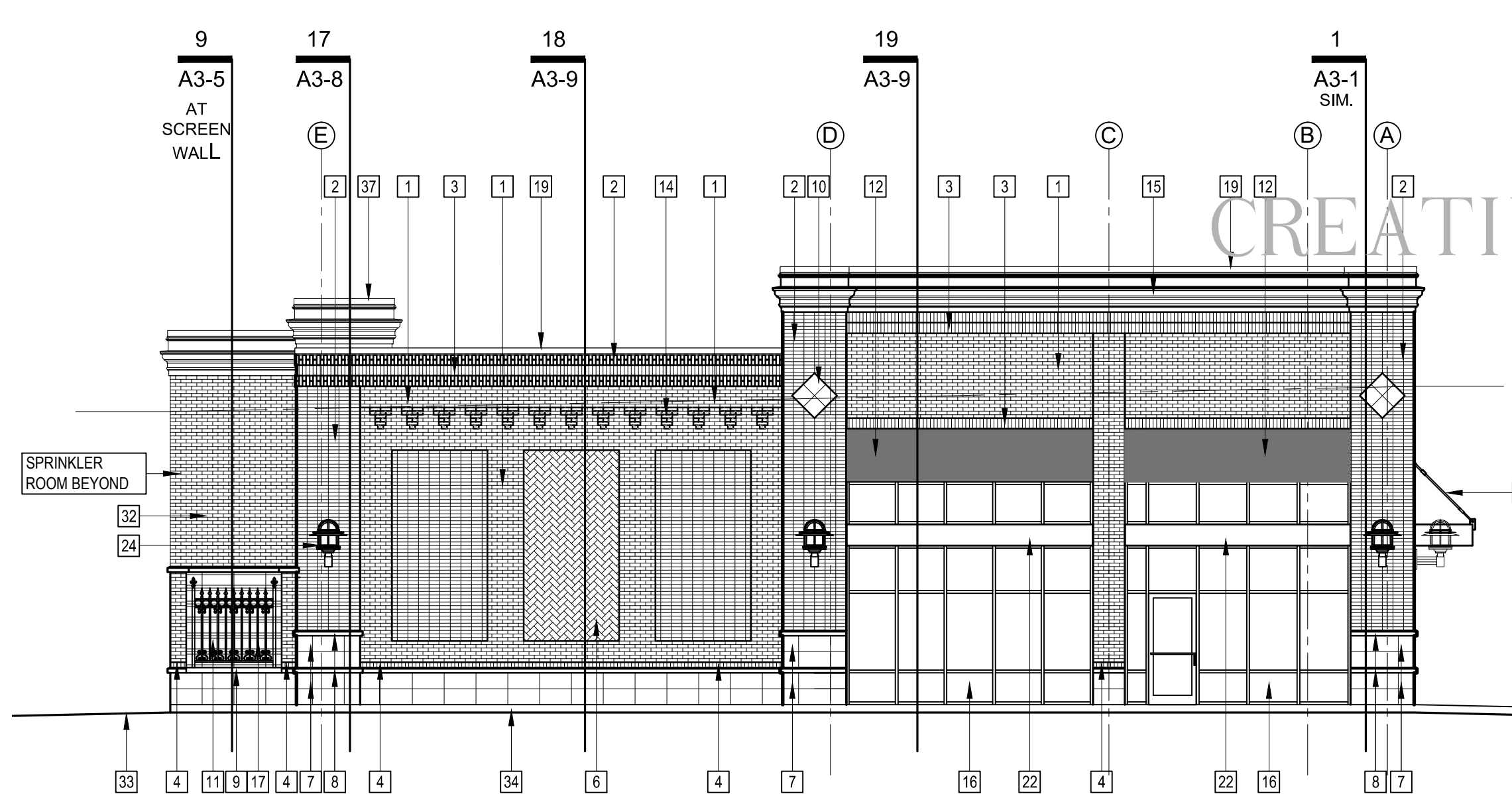
3 BUILDING A SOUTH ELEVATION 1/8"=1'-0"
