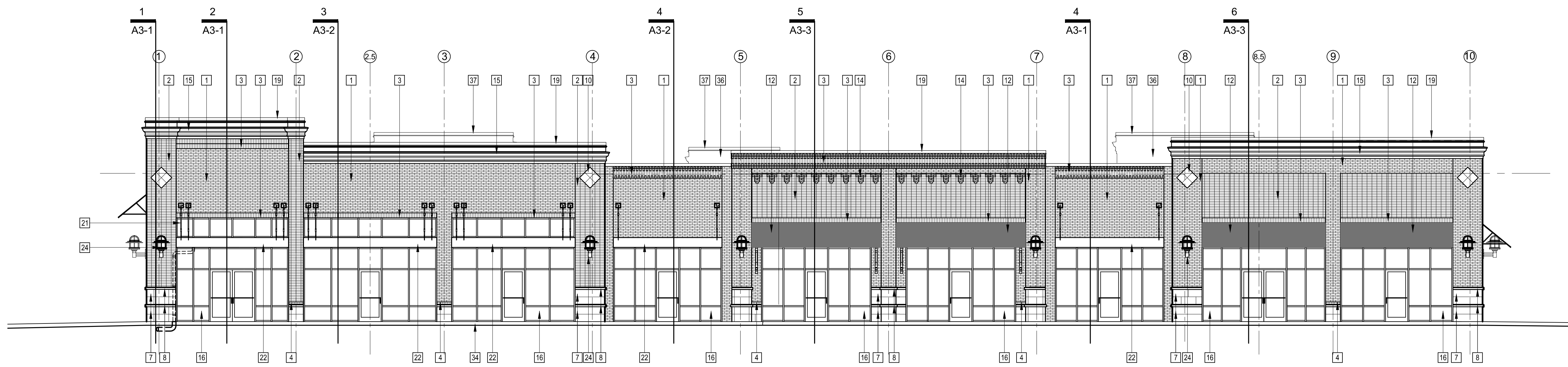
1 BUILDING A EAST ELEVATION 1/8"=1'-0"
