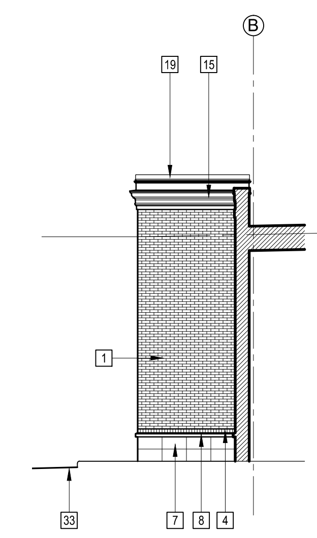
5 SPRINKLER RISER RM. BLDG A SOUTH ELEVATION 1/8"=1'-0"
