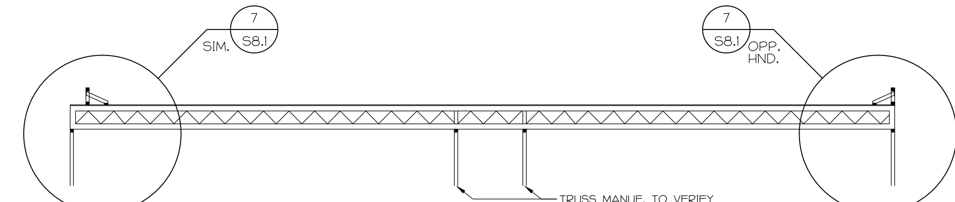
12 TRUSS DIAGRAM S8.3 1/8" = 1'-0"
