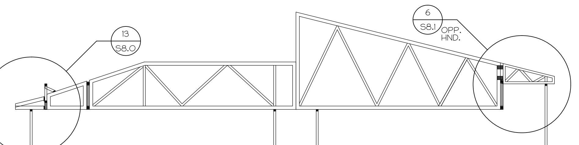
4 TRUSS DIAGRAM S8.3 1/8" = 1'-0"
