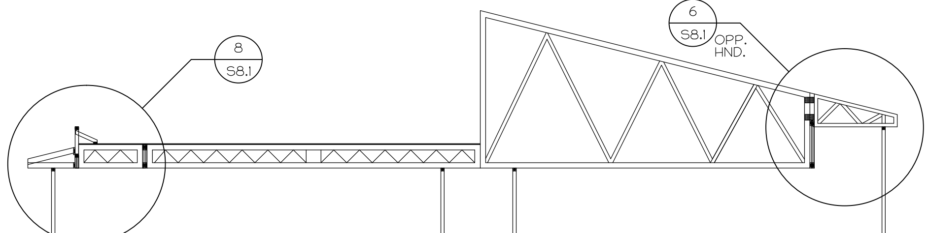
8 TRUSS DIAGRAM S8.3 1/8" = 1'-0"
