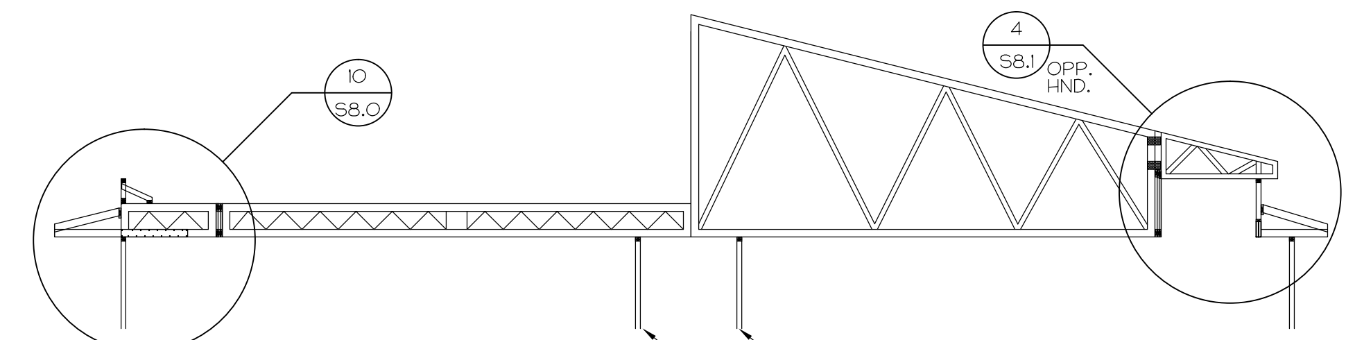
11 TRUSS DIAGRAM S8.3 1/8" = 1'-0"
