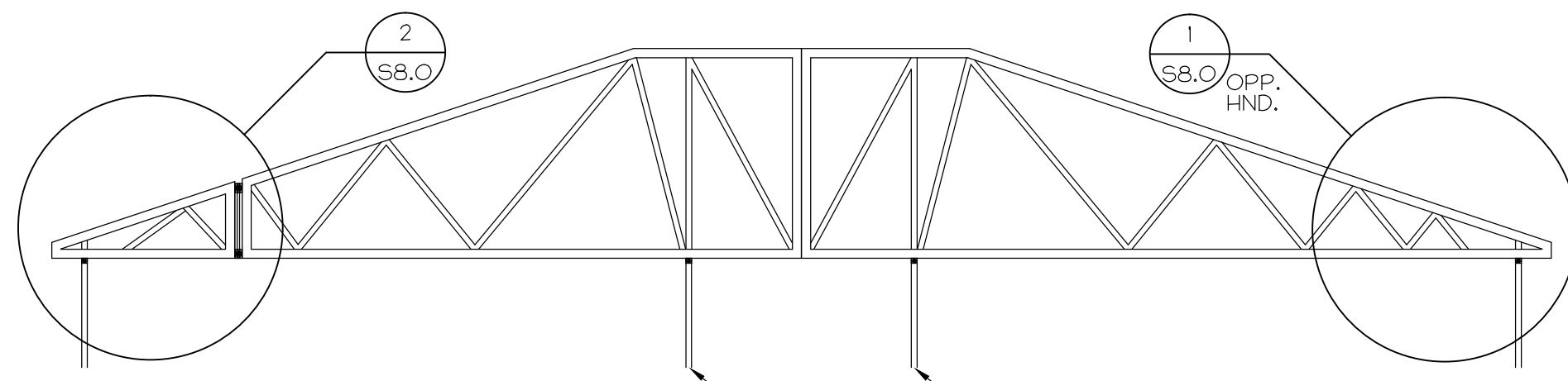
1 TRUSS DIAGRAM S8.3 1/8" = 1'-0"
