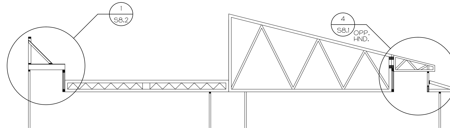
6 TRUSS DIAGRAM S8.3 1/8" = 1'-0"
