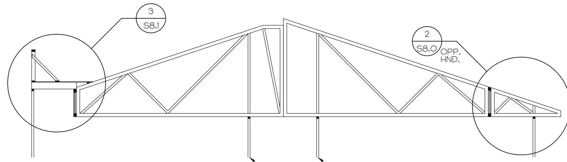
1 TRUSS DIAGRAM S8.3 1/8" = 1'-0"
