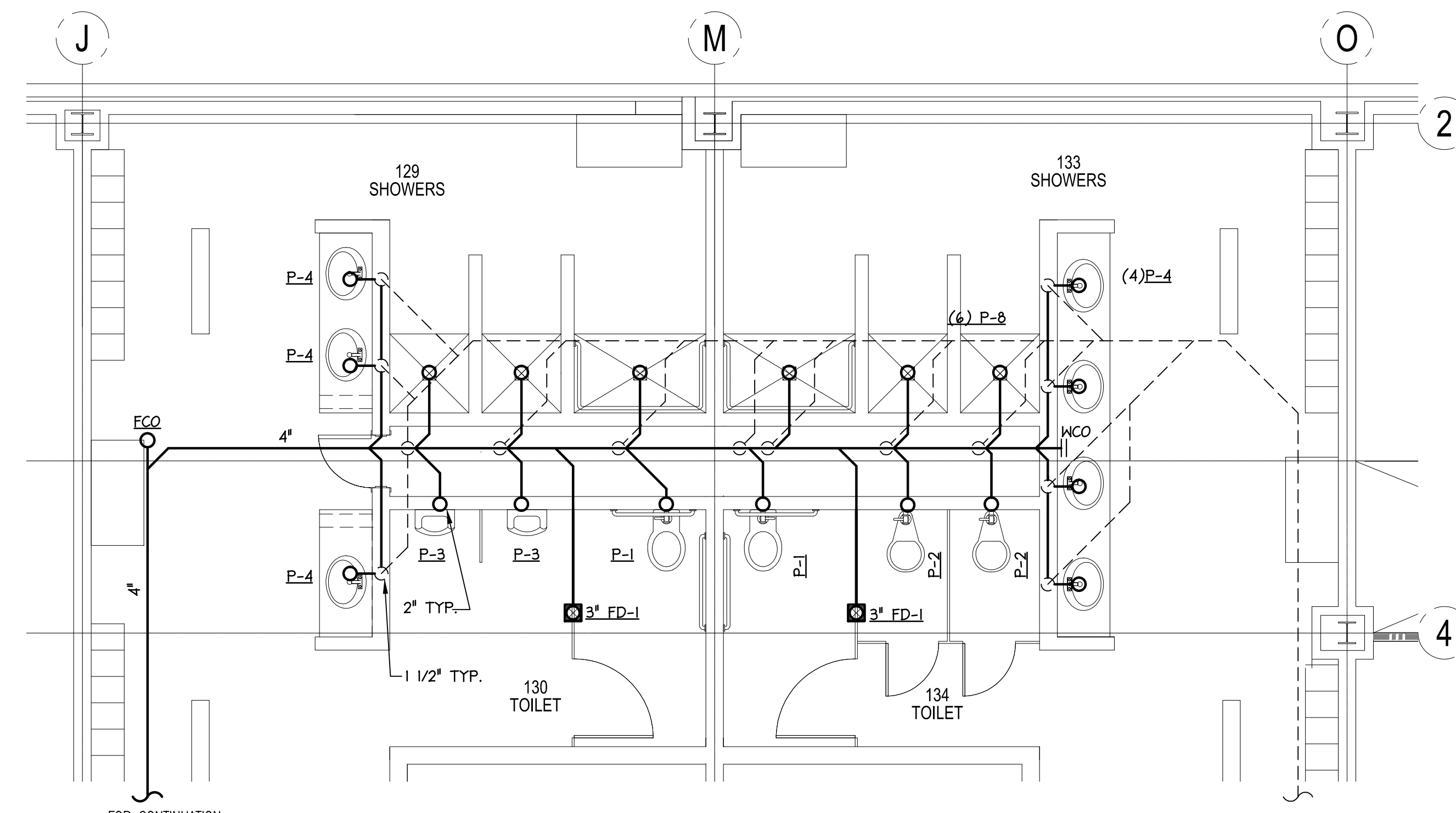
2 ENLARGED 1ST FLOOR SANITARY PLAN 1/4" = 1'-0"
