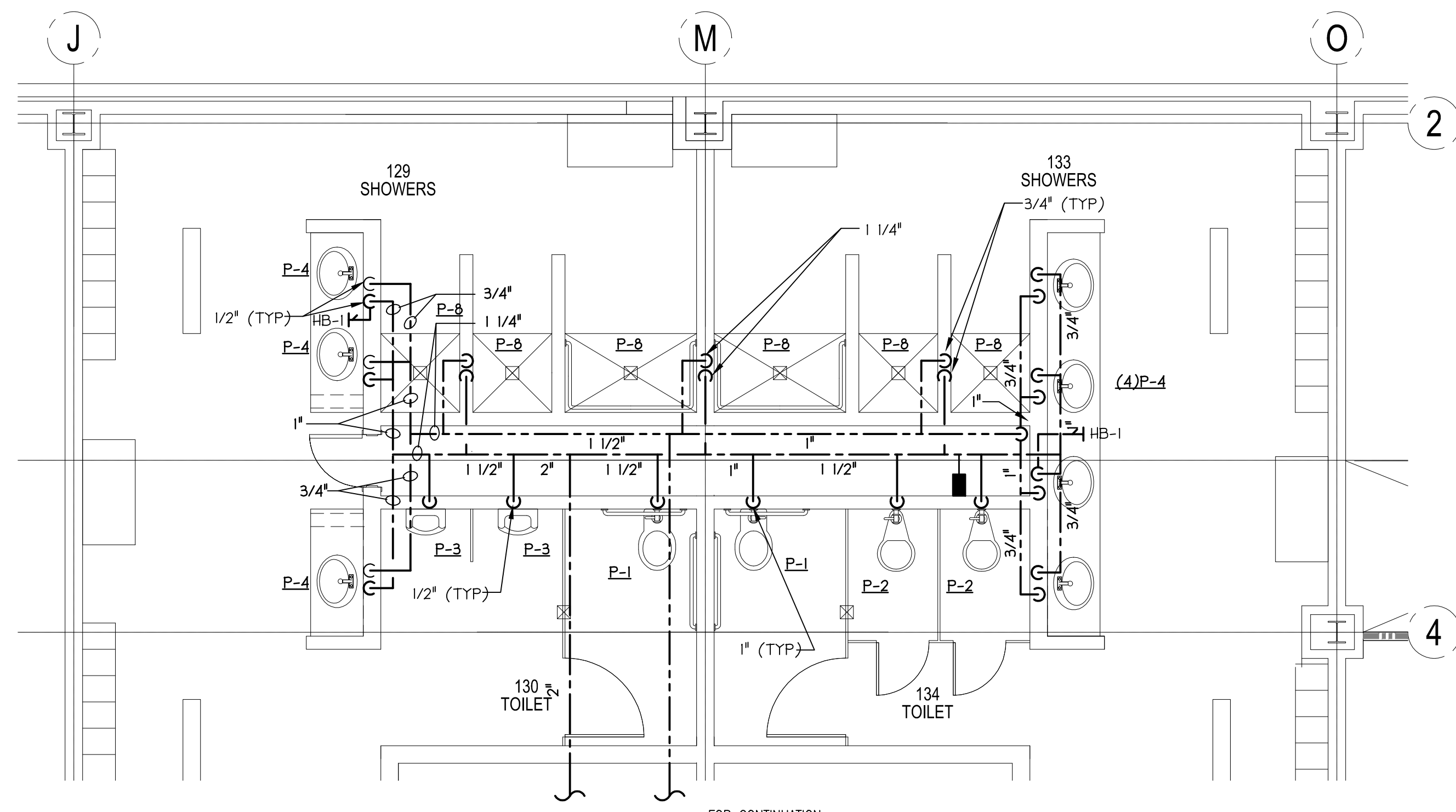
1 ENLARGED 1ST FLOOR DOMESTIC WATER PLAN 1/4" = 1'-0"
