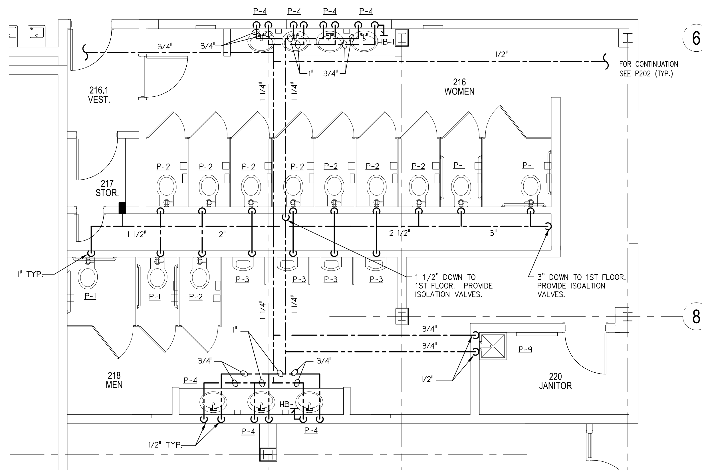
5 ENLARGED 2ND FLOOR DOMESTIC WATER PLAN 1/4" = 1'-0"
