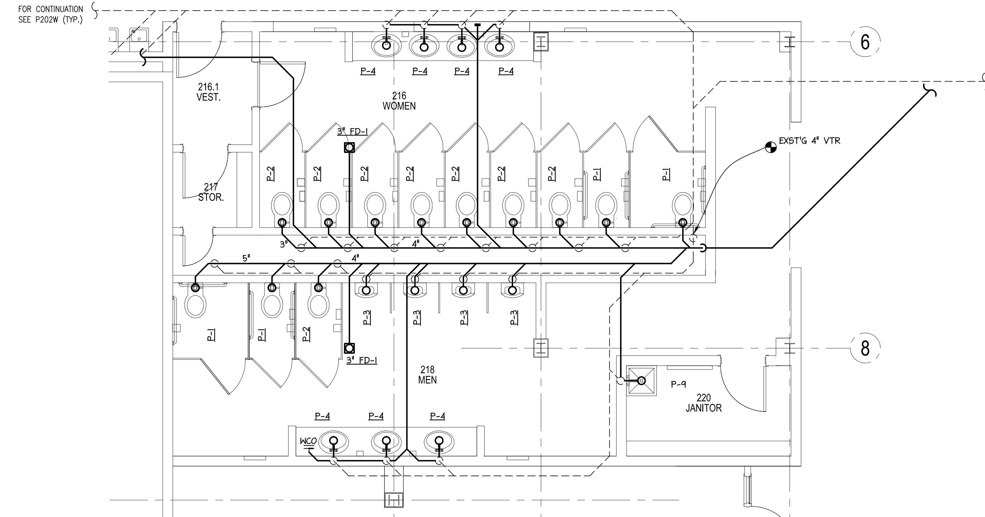
6 ENLARGED 2ND FLOOR SANITARY PLAN 1/4" = 1'-0"
