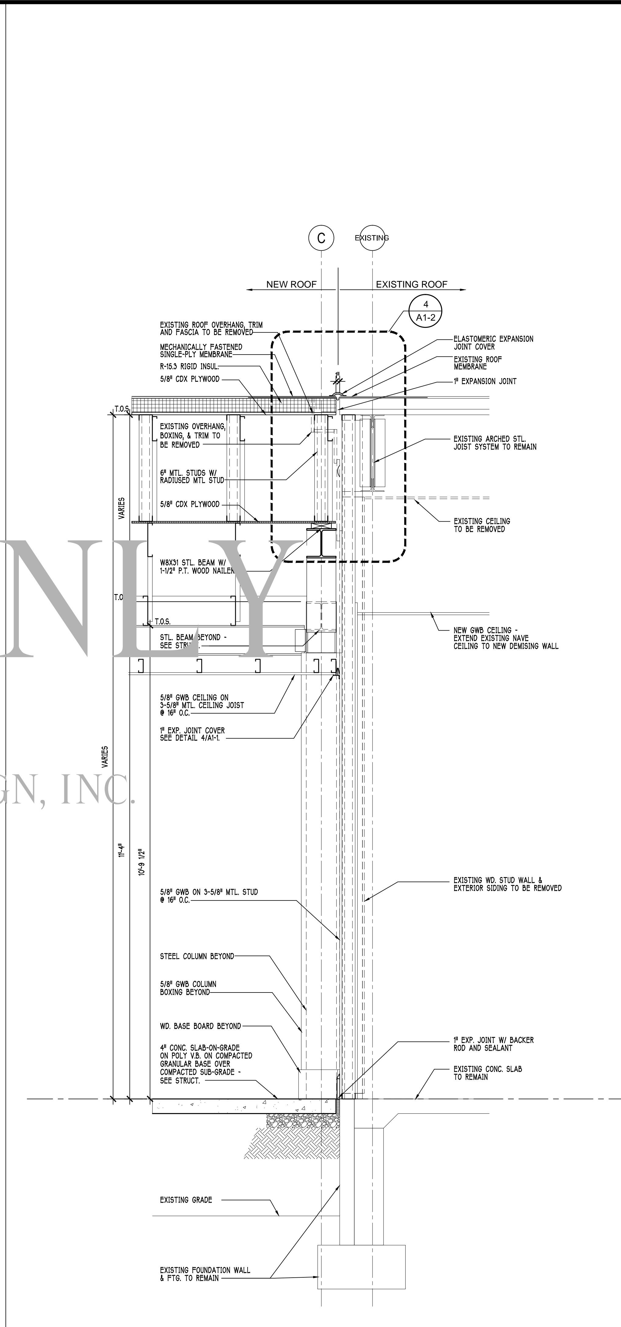
4 WALL SECTION
